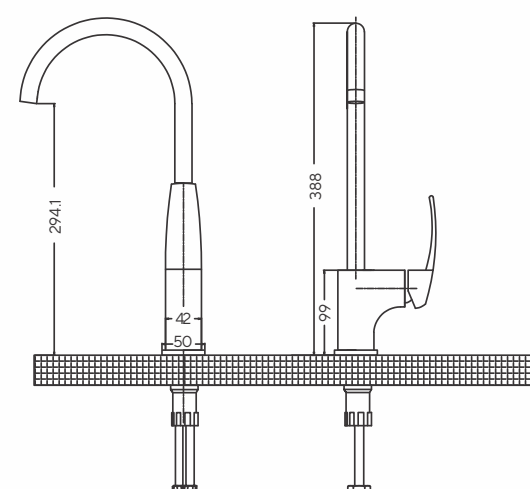
Q253118120 Marsala Single Function Deck-Mount Kitchen Faucet MRP: ₹ 15,990
