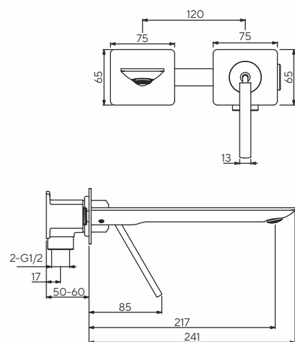
Q913100224 Single Control Wall Mount Basin Mixer Trim & Diverter in Matt Black MRP: ₹ 41,990
