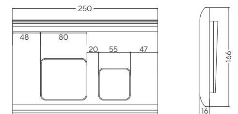
Q507455120 Sisma Flush Plate MRP: ₹ 1,890
