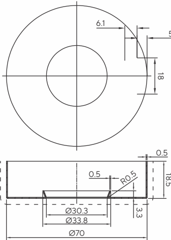
Q503200320 Ceiling Shower Arm (Brass) Round 150mm in Polished Chrome MRP: ₹ 3,490
