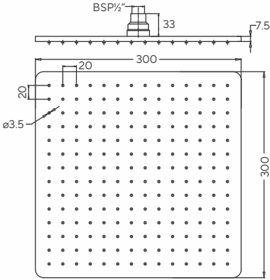
Q503146220 Overhead Shower 300x300mm in Chrome MRP: ₹ 15,990
